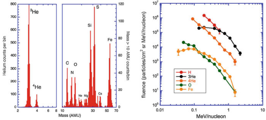
Fig. 4.16 Mass histograms of the 16 May 2014 ^3\text{He} -rich event are shown in the left two panels and some corresponding energy spectra are shown in the right panel (Mason et al. 2016)
