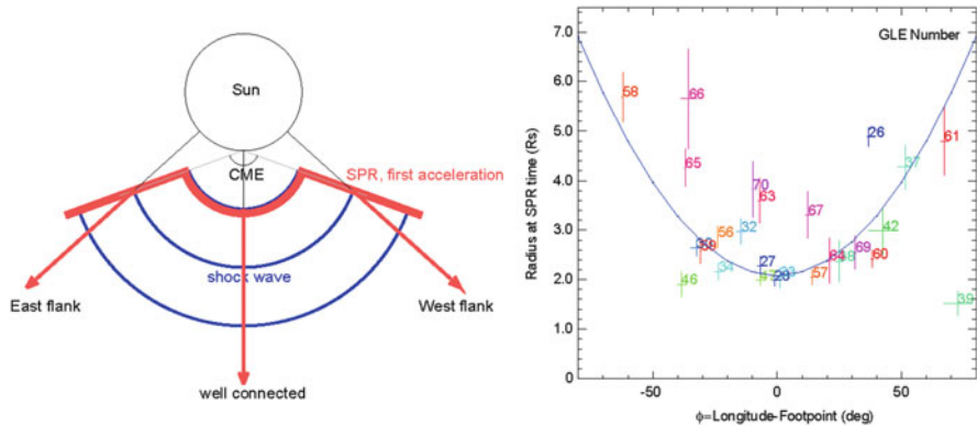
Fig. 3.3 The right panel shows the height of the CME at SPR time vs. longitude for numbered GLEs. The cartoon on the left shows the CME and SPR location widening on the flanks (Reames 2009a, b). The height distribution has been fit to a symmetric parabola for comparison; actually a height of 2–3 R_S is fairly constant over \sim 70^\circ . This could be the width of the source shock surface above closed loops that was once incorrectly called the “fast propagation region”
