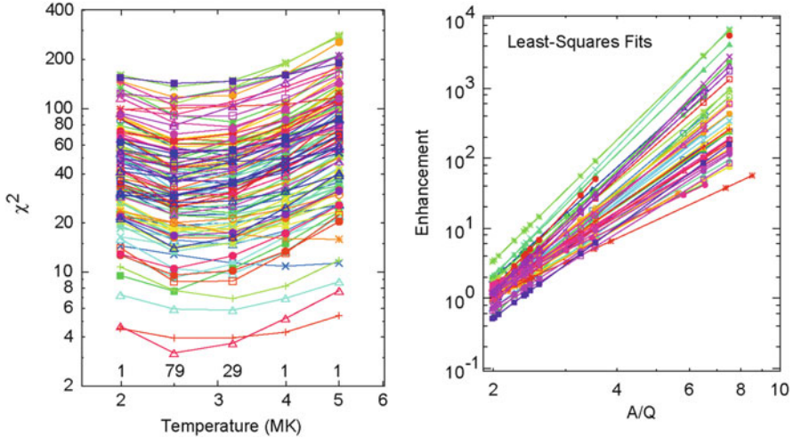
Fig. 4.10 The left panel shows \chi^2 versus T for all 111 impulsive SEP events using different colors and symbols for each event. The number of events with \chi^2 minima at each temperature is shown along the bottom of the panel. The right panel shows the distribution of the fits (Reames et al. 2014b)
