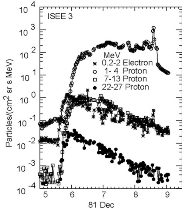
Fig. 2.10 Intensities vs. time are shown for the disappearing-filament-associated SEP event of 5 December 1981. The peak in the low energy protons on 8 December occurs at the time of shock passage at 1 AU
