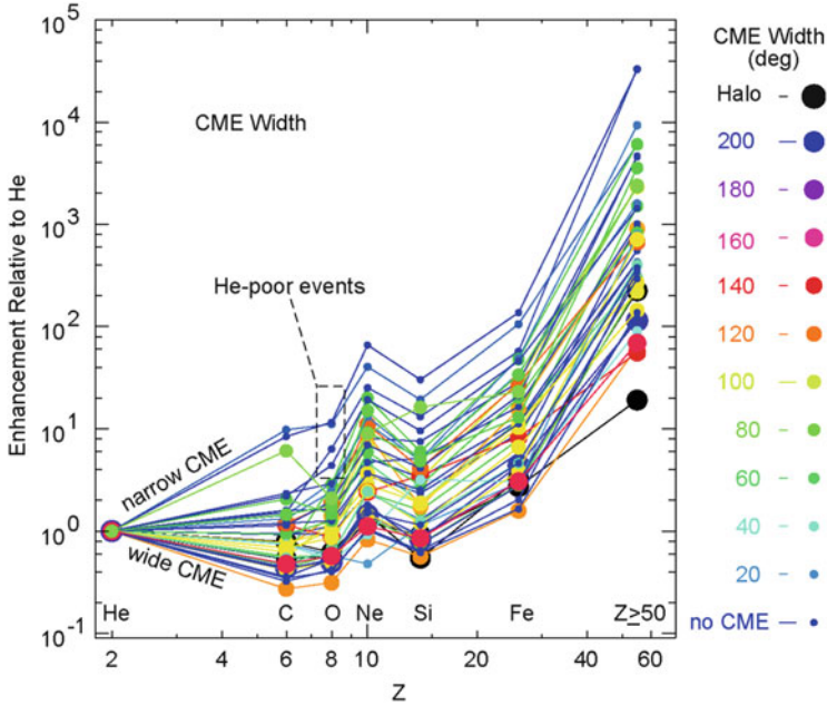
Fig. 4.12 Enhancements relative to He are shown versus Z for impulsive SEP events. Symbol sizes indicate the associated CME width (Reames et al. 2014a)
