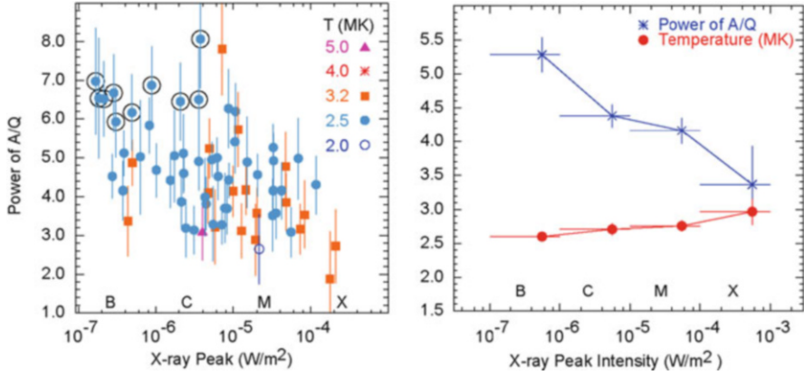
Fig. 4.13 The left panel shows the power of A/Q versus the GOES soft X-ray peak intensity (and “CMX” class) for individual SEP events with temperature as a symbol and color . Circled events are “He-poor” with low {}^4\text{He}/\text{O} caused by increased A/Q for O. The right panel shows variation of the mean temperature and power of A/Q within each soft X-ray class (after Reames et al. 2014b)
