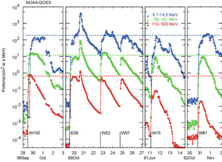
Fig. 6.5 Intensity levels are shown in six large SEP events with the corresponding streaming limit (Reames and Ng 1998)
