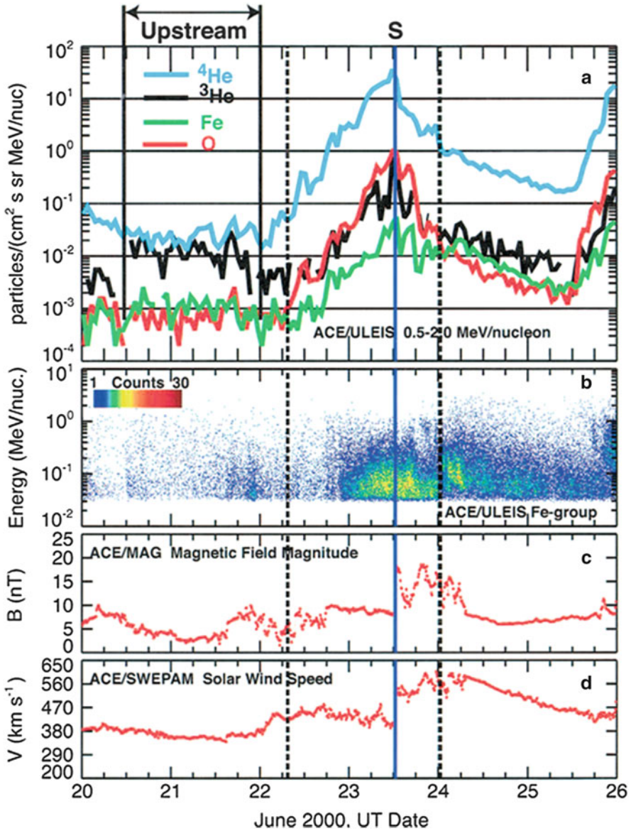
Fig. 2.7 (a) Intensities of 0.5–2.0 MeV \text{amu}^{-1} ^3\text{He} , ^4\text{He} , O and Fe are shown during a large SEP event, with (b) a histogram of Fe arrivals, (c) the magnetic field B, and (d) the solar wind speed. ^3\text{He} is clearly accelerated, peaking at the shock, S, but is not as strongly enhanced as in the ^3\text{He} -rich period upstream (Desai et al. 2003; see also Bućik et al. 2014, 2015; Chen et al. 2015)
