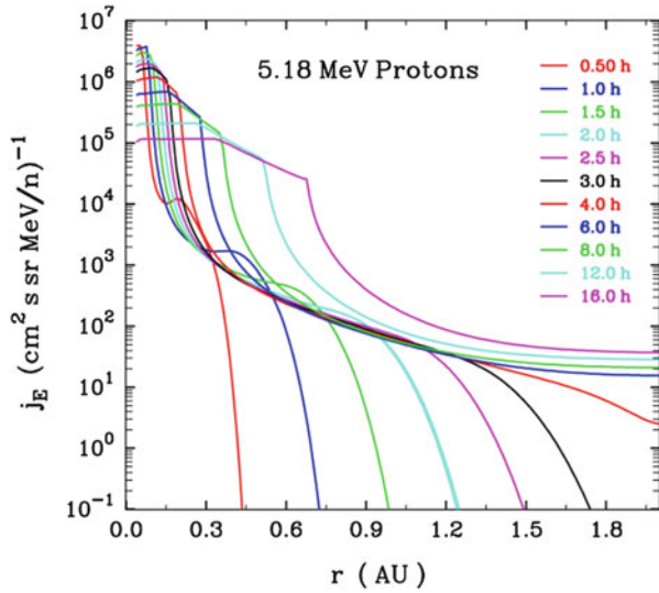
Fig. 6.7 Theoretical intensity of 5.18 MeV protons versus radius is shown as it varies with time during a large SEP event. Soon after arrival at a given radius, intensities rise to the streaming limit at that radius. At 1 AU, intensities are bounded near \sim 100 \text{ (cm}^2 \text{ s sr MeV/n)}^{-1} until the shock reaches \sim 0.7 \text{ AU} (Ng et al. 2003, 2012)
