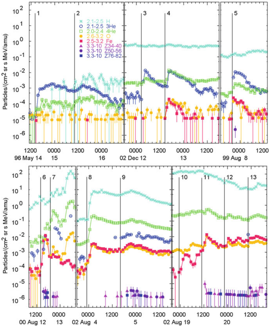
Fig. 4.2 Intensities of H, {}^3\text{He} , {}^4\text{He} , O, Fe, and heavy elements are shown as a function of time during 13 impulsive SEP events (Reames and Ng 2004)
