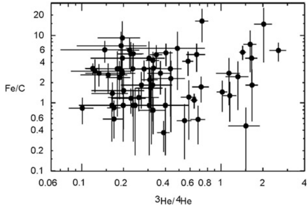
Fig. 4.5 Cross plots of Fe/C versus {}^3\text{He}/{}^4\text{He} at 1.3–1.6 MeV \text{amu}^{-1} in impulsive SEP events shows little evidence of correlation (Reames 1999; adapted from Reames et al. 1994)
