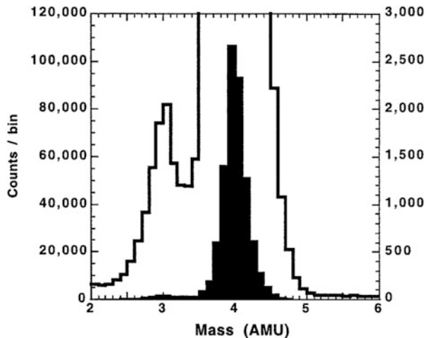
Fig. 2.6 The mass distribution of He is shown directly ( solid —left scale) and with an expanded scale ( open —right scale) to show ^3\text{He} at 0.2–2.0 MeV \text{amu}^{-1} during quiet times (Mason et al. 1999)
