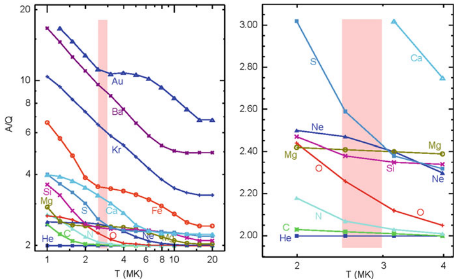
Fig. 4.8 A/Q is shown as a function of equilibrium temperature for various elements (left panel) and is enlarged for low Z (right panel). Elements below Fe are from Arnaud and Rothenflug (1985), Fe from Arnaud and Raymond (1992) and sample elements in the high- Z region from Post et al. (1977). The region used for Fe-rich impulsive SEP events is shaded
