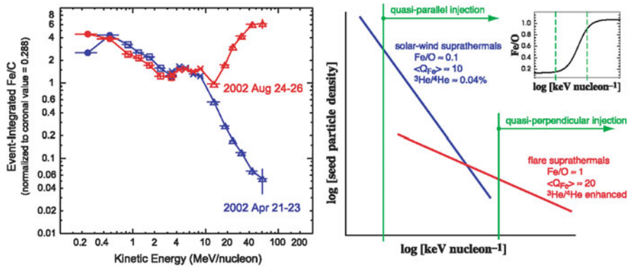
Fig. 2.8 The left panel compares the energy dependence of Fe/C for two gradual events that are otherwise similar in their properties (Tylka et al. 2005). The right panel shows hypothetical spectra of two sources of suprathermal ions where different injection thresholds will yield different abundance ratios (Tylka et al. 2005). Clearly, it would be unwise to use measurement of Fe/C above \sim 10 MeV \text{amu}^{-1} in an attempt to distinguish impulsive and gradual SEP events
