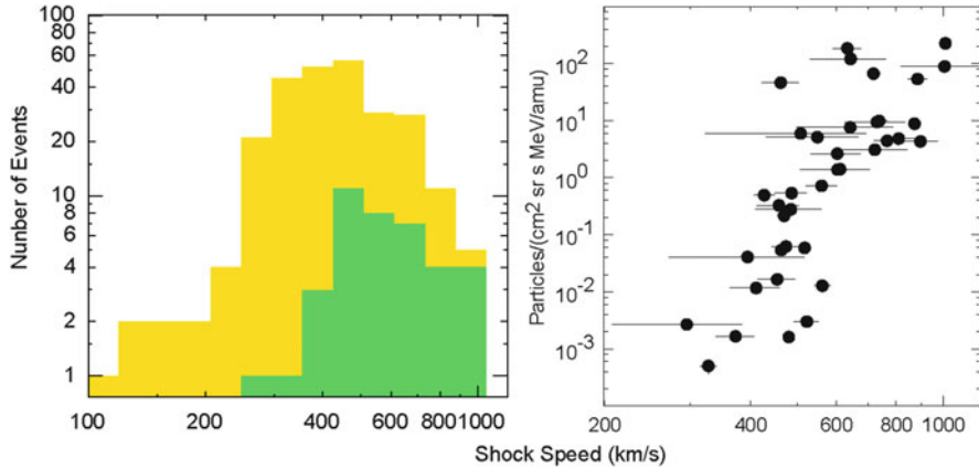
Fig. 5.9 The left panel shows the distribution of shock waves at 1 AU with measurable acceleration of >1 \text{ MeV amu}^{-1} \text{ He} vs. shock speed ( green ) within the distribution of all 258 shock waves vs. shock speed ( yellow and green ) observed by the Wind spacecraft. The right panel shows the background-corrected peak intensity of 1.6\text{--}2.0 \text{ MeV amu}^{-1} \text{ He} vs. shock speed for the shocks in situ. Shock speed is the strongest determinant of accelerated intensity for local shocks; this mirrors the correlated behavior of peak intensity vs. CME speed in Fig. 2.11 (adapted from Reames 2012, 2013)
