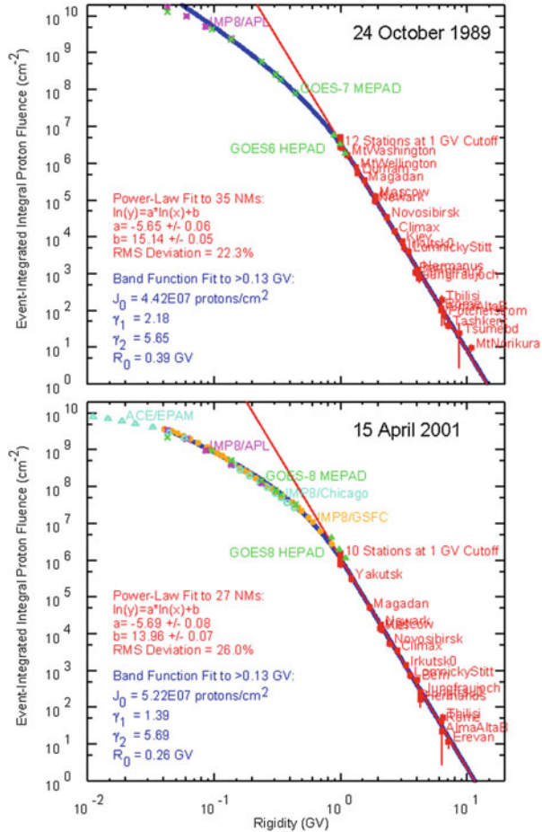
Fig. 6.2 Integral rigidity spectra are shown for two large GLEs. Cutoff rigidities for individual neutron-monitor stations (listed) are used; the spectra are corrected for neutron production versus proton energy, and compared with the named satellite measurements. Fits to double power-law (Band) spectra are shown (Tylka and Dietrich 2009)
