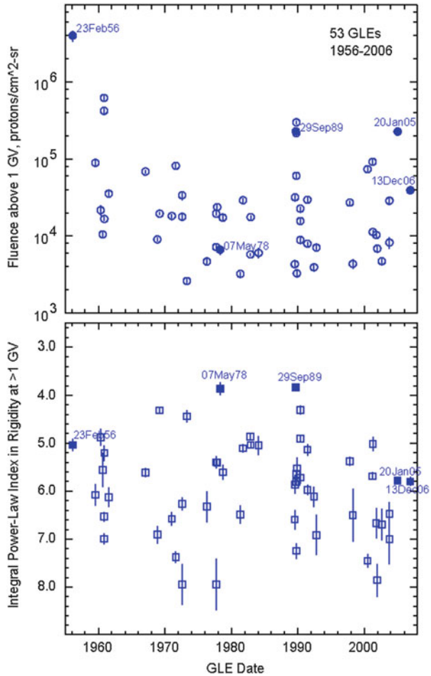
Fig. 6.3 The upper panel shows the proton fluence above 1 GV (430 MeV) versus time for each GLE. The lower panel shows the integral rigidity power-law spectral index also above 1 GV (Tylka and Dietrich 2009)
