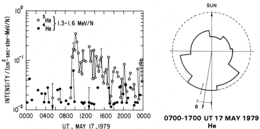
Fig. 2.5 Intensities of ^3\text{He} and ^4\text{He} (left) and ^3\text{He} angular distribution (right) in a small ^3\text{He} -rich event associated with 2–100 keV electrons (Reames et al. 1985)
