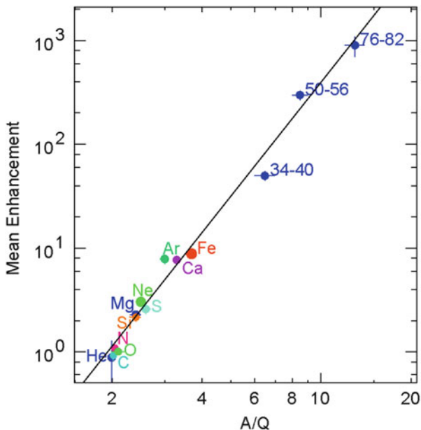
Fig. 4.9 The mean enhancement in the abundances of elements in impulsive SEP events relative to reference gradual events is shown as a function of A/Q of the element. For the least-squares fit line shown in the figure the enhancement varies as the 3.64 \pm 0.15 power of A/Q (Reames et al. 2014a)
