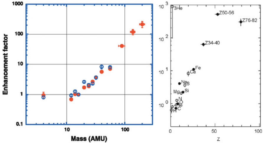
Fig. 4.7 Enhancements relative to solar system and coronal abundances are extended to high masses at 0.1–1.0 MeV \text{amu}^{-1} in the left panel (red, Mason et al. 2004) and to high Z at 3.3–10 MeV \text{amu}^{-1} in the right (Reames and Ng 2004). Open symbols are from Reames (1995)
