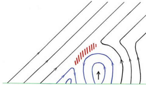
Fig. 4.14 A jet is produced when newly emerging magnetic flux ( blue ) reconnects with open field lines ( black ) in the red shaded region. Energetic particles and plasma can escape toward the upper right (Reames 2002)
