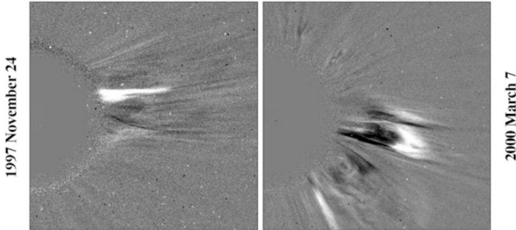
Fig. 4.15 Difference images show the change in intensity in the LASCO C2 coronagraph for the narrow CMEs associated with two impulsive SEP events (Kahler et al. 2001)
