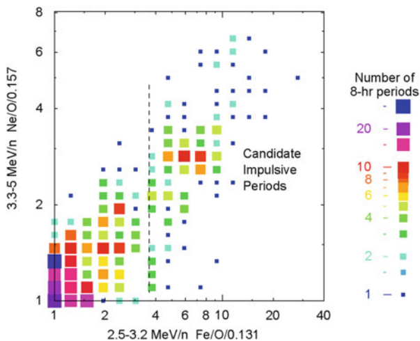
Fig. 4.1 Measured relative enhancements in \text{Ne}/\text{O} versus \text{Fe}/\text{O} for 8-h periods during 19 years are binned for all periods with errors of 20% or less (Reames et al. 2014a)
