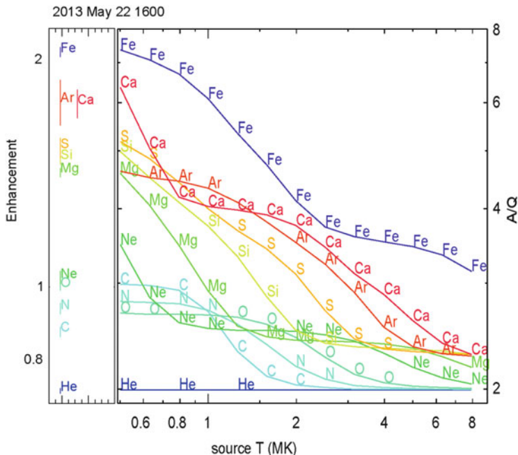
Fig. 5.12 The left panel shows the abundance enhancements at \sim 3\text{--}5 \text{ MeV amu}^{-1} observed early in the 22 May 2013 SEP event. The right panel compares a section of the A/Q vs. T plot from Fig. 5.11. The patterns match at about 0.6 MK (Reames 2016a)
