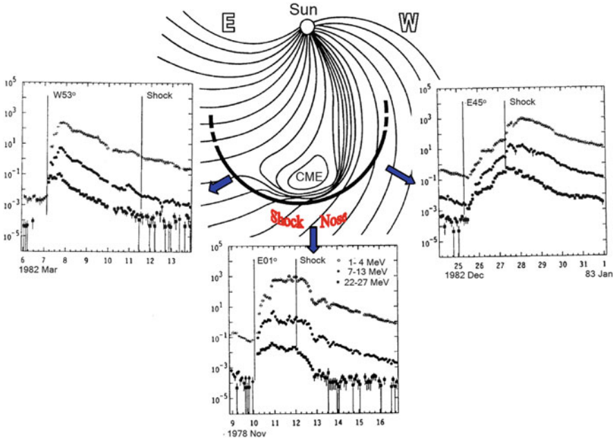
Fig. 2.1 Variation of the appearance of typical SEP events is shown as viewed from three solar longitudes (see text; after Reames 1999; see also Cane et al. 1988)
