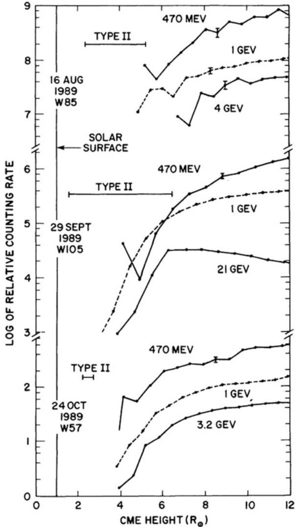
Fig. 3.6 Injection profiles of high-energy protons are shown as a function of CME height for three GLEs in 1989: August 16, September 29, and October 24. The CME speeds for these events are 1377, 1828, and 1453 km s -1 , respectively (Kahler 1994)
