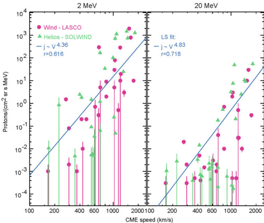
Fig. 2.11 Peak intensity is shown vs. CME speed for 2 MeV ( left ) and 20 MeV ( right ) protons for two event samples (see text). Power-law least-squares fits and correlation coefficients ( r ) are shown (see Kahler 2001)
