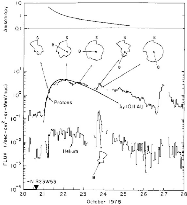
Fig. 2.2 Intensities and angular distributions of \sim 1 MeV \text{amu}^{-1} H and He are shown for a large SEP event of 21 October, 1978 and for the newly anisotropic flow from a small {}^3\text{He} -rich event on 23 October. A diffusion fit, to the proton intensity is shown with a radial component of the scattering mean free path of 0.11 AU. How can scattering spread particles in time so much in the large event, but barely scatter those from the small event in its wake? (Mason et al. 1989)
