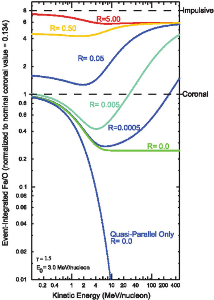
Fig. 2.9 The energy dependence of Fe/O is shown as a function of R which is the ratio, in the seed population, of O in impulsive suprathermal ions to coronal ions. The values of \gamma and E_0 assumed for this case are shown in the lower left corner of the figure (Tylka and Lee 2006)
