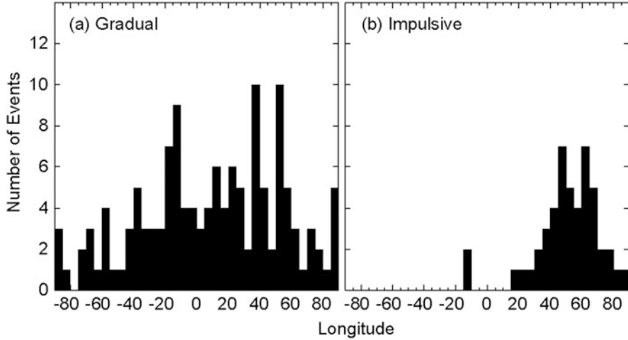
Fig. 2.3 Longitude distributions are shown for gradual SEPs ( left ) spread mainly because of the width of the shock source, and impulsive ( right ) SEP events spread by random walk of field lines and by variations in solar wind speed (Reames 1999)
