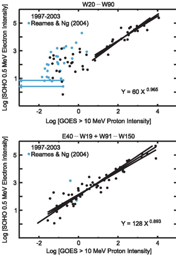
Fig. 3.9 The panels each show peak 0.5 MeV electron intensity vs. peak 10 MeV proton intensity. Events in the upper panel are well connected (20–90 W) while those in the lower panel are poorly connected. The events in blue are impulsive events that are ^3\text{He} -rich with enhanced heavy elements. A proton-intense subset of well-connected events shows a strong correlation while essentially all of the poorly-connected events are correlated (Cliver and Ling 2007)
