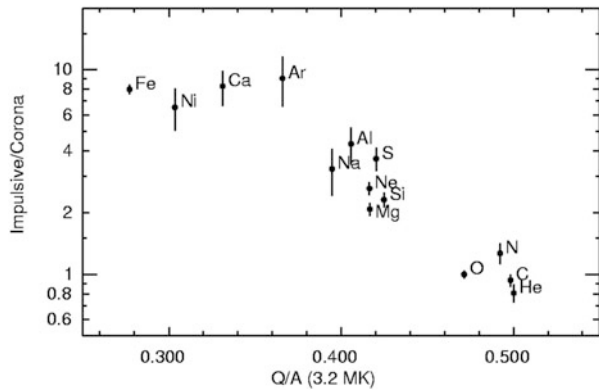
Fig. 4.6 Average abundance enhancements of elements in impulsive SEP events versus Q/A at 3.2 MK as of 1995 as shown by Reames (1999)
