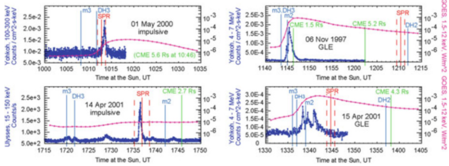
Fig. 3.2 A comparison is shown of timing in two impulsive ( left ) and two gradual ( right ) SEP events. Solar particle release (SPR) times of the particles ( red with dashed errors ) are compared with hard X-ray ( dark blue, left ), \gamma -ray ( dark blue, right ) and GOES soft X-ray ( violet ) time profiles. Onset times of metric (m) and decametric-hectometric (DH; 1–14 MHz) type II and III radio bursts ( light blue ) and CME locations ( green ) are shown (adapted from Tylka et al. 2003)
