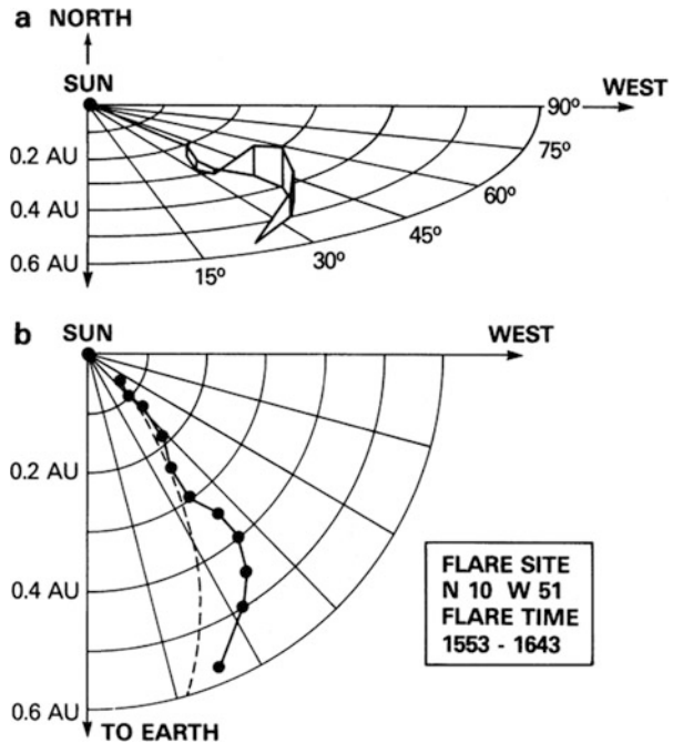
Fig. 3.10 The trajectory of the electron population in the type III radio burst accompanying a ^3\text{He} -rich SEP event is shown in three dimensions (a) and as a projection on the ecliptic (b) (Reames and Stone 1986)
